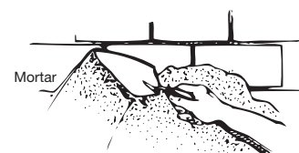
Figure 6 Apply mortar using a mason's trowel.
